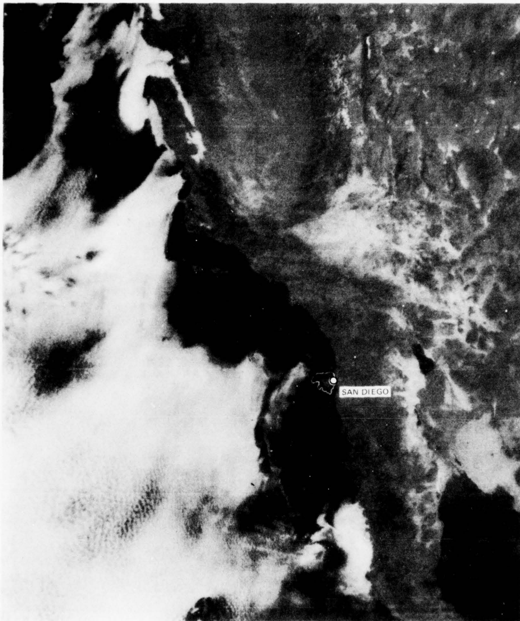
Figure 14. Enlargement of DMSP image at 0852 PDT on 8 October 1976. (Fog area outlined in white for reader's convenience.)
